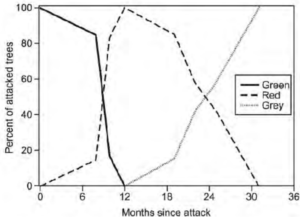
Fig. 1. Variability in fading rate of foliage within a sample lodgepole pine stand (Fountain Valley Site 2, Kamloops Forest District, between 1962 and 1965) post-mass-attack. This example stand was composed of 15 attacked trees.
